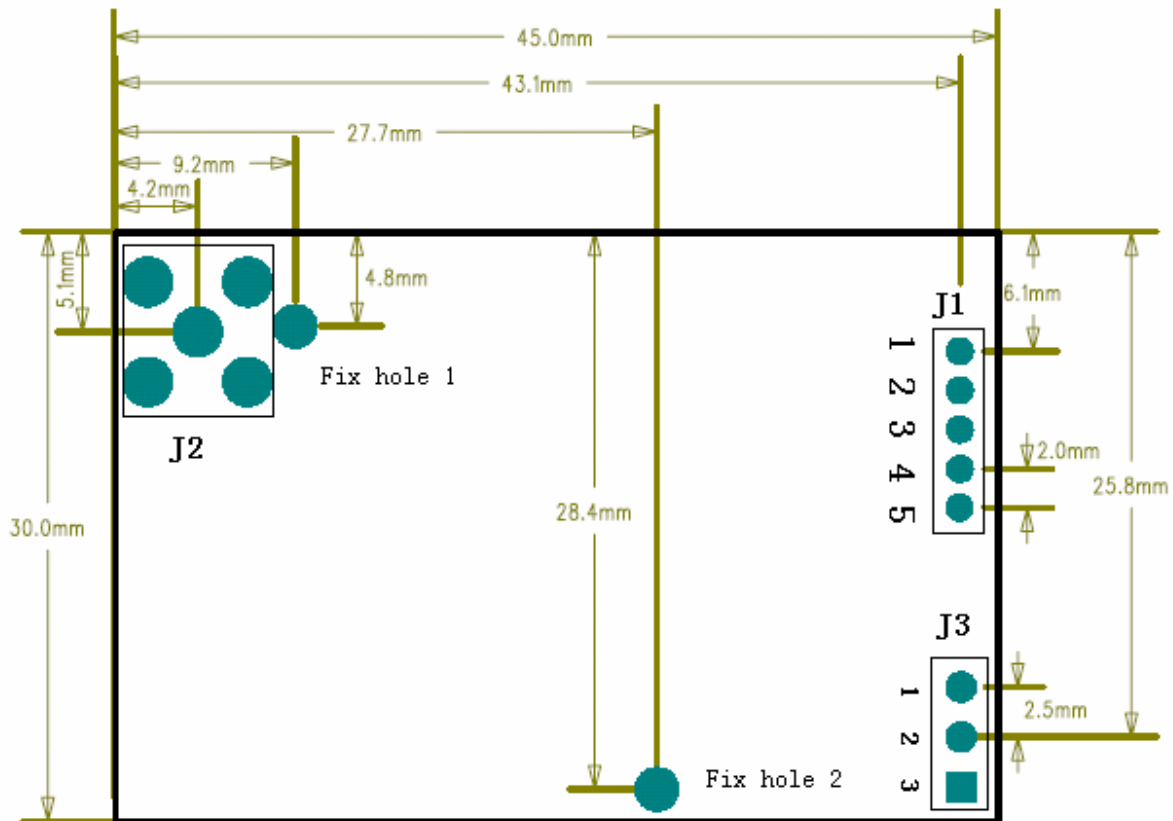
Fig1. FC-211SP Interface sketch map(View from the back of PCB v4.1)
