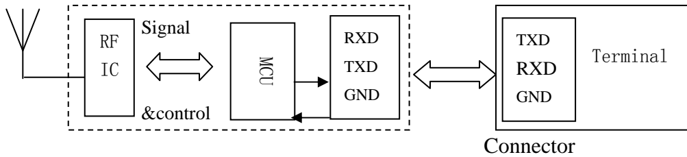
Fig2.FC-211SP application principle map
